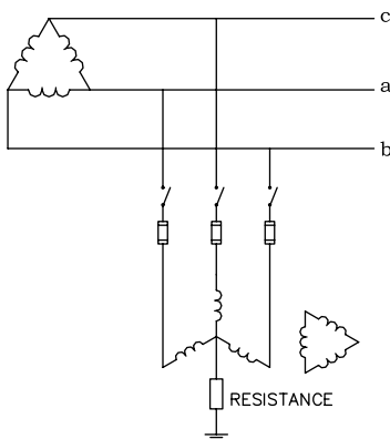
7a – LOW VOLTAGE SYSTEM
