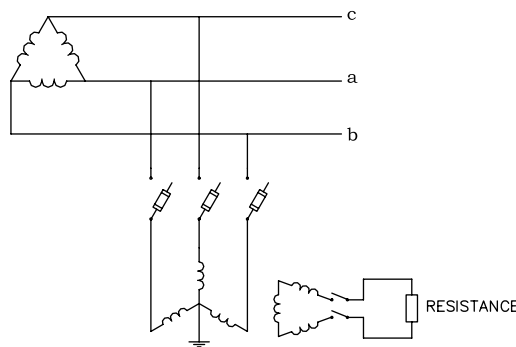
7b – MEDIUM VOLTAGE SYSTEM
