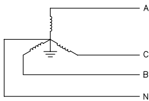
SOLIDLY GROUND 4 WIRE SYSTEM USE THREE ELEMENT CONNECTION
