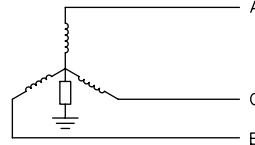
IMPEDANCE GROUND WYE SYSTEM NORMAL CONNECTION: TWO ELEMENT SPECIAL CONNECTION: THREE ELEMENT
