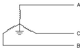
SOLIDLY GROUND 3 WIRE SYSTEM USE TWO ELEMENT CONNECTION
