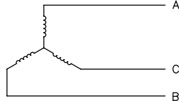
UNGROUND WYE SYSTEM NORMAL CONNECTION: TWO ELEMENT SPECIAL CONNECTION: THREE ELEMENT
