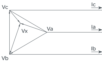
Figure 2: Blondel theorem
